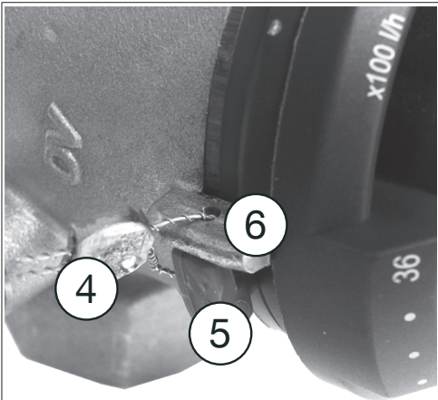
Fig. 12: Securing of the presetting
