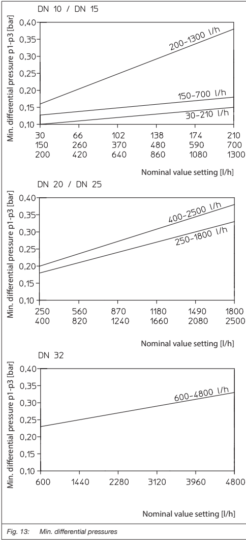
Fig. 13: Min. differential pressures
