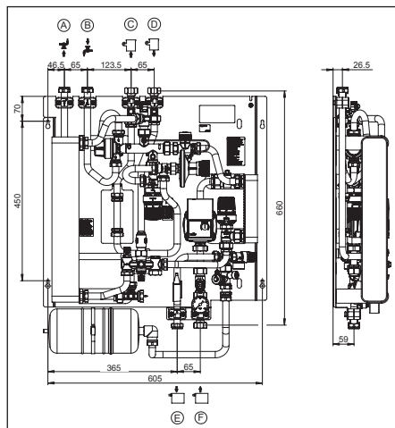
Illustr. 2 Dimensions
