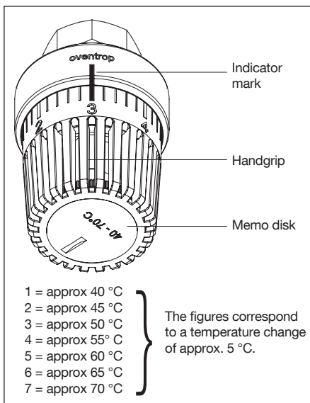
Illustr. 4 Setting of the potable water temperature
