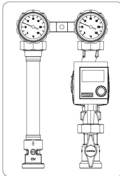
Regumat S-180 - reduced dimensions
