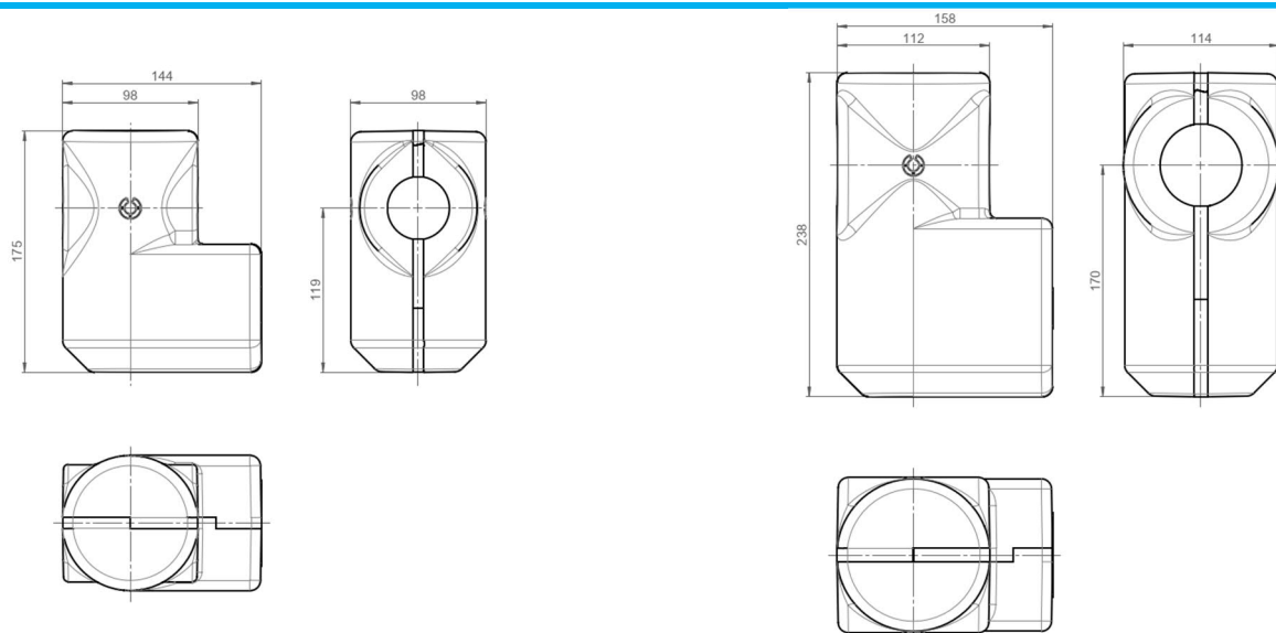
For DN 20 and DN 25, for horizontal installation position (item no. 1124091)
