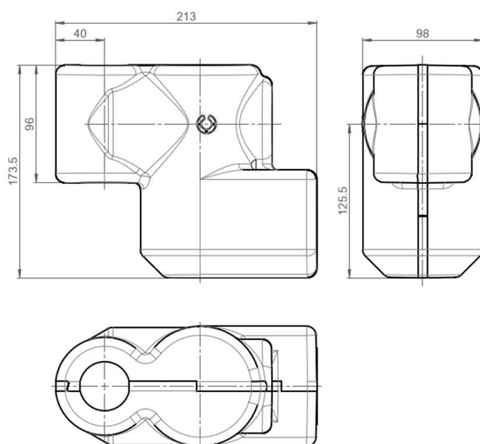
For DN 20 and DN 25, for vertical installation position (item no. 1124191)
