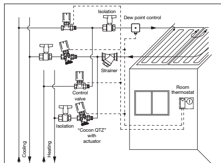
Illustr. 6.2 Four pipe system
