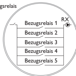
1. Parallel (OR)
