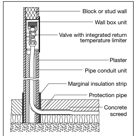
Cut
