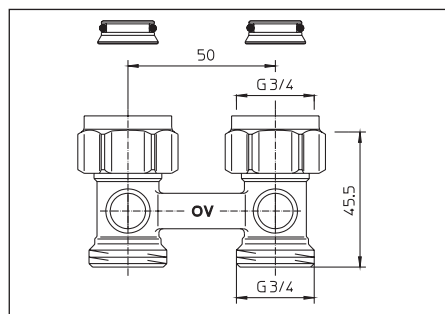
Illustr. 4 Straight pattern, G 3/4 collar nut x G 3/4 male thread
