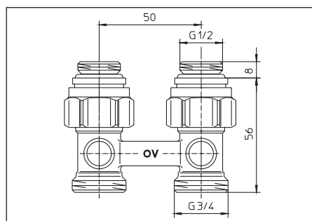
Illustr. 5 Straight pattern, G 1/2 male thread x G 3/4 male thread
