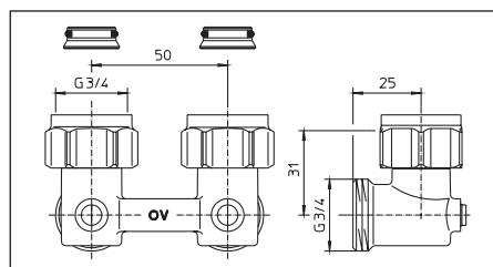
Illustr. 6 Angle pattern, G 3/4 collar nut x G 3/4 male thread
