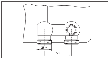
Illustr. 9 Distributor with G 3/4 male thread according to DIN EN 16313 (cone "Euro")
