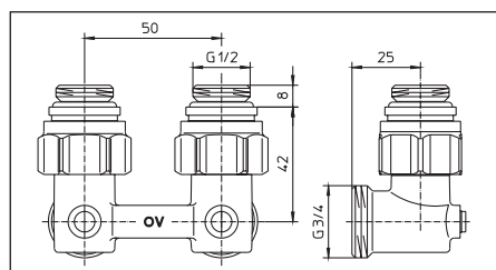
Illustr. 7 Angle pattern, G 1/2 male thread x G 3/4 male thread
