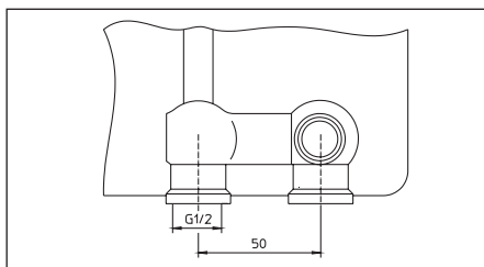
Illustr. 8 Distributor with G 1/2 female thread
