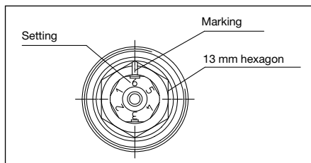
Illustr. 6.2 Presettable valve insert
