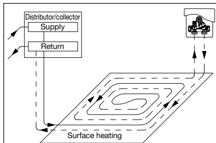
Illustr. 5.3 Installation sketch
