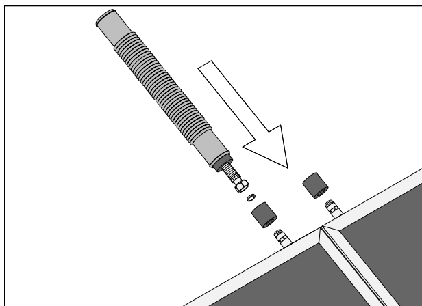
Illustr. 3 Installation of collector coupling hose: Slide short pipe insulation onto the connection nipples, mount pre-assembled corrugated hose with gasket and slightly tighten by hand.
