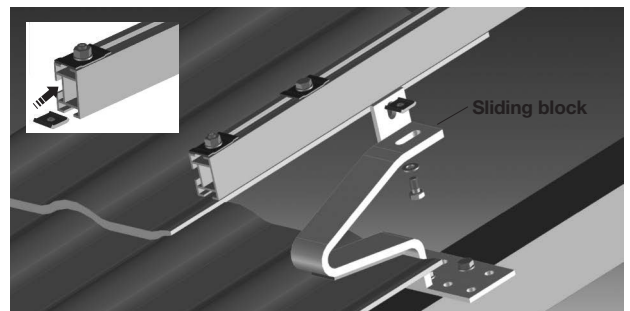
Illustr. 7: Fitting of mounting rails
