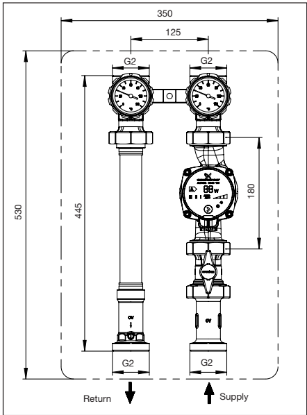
Pump group "Regumat S-180"
