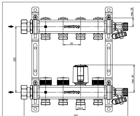
Illustr. 5: Dimensions
