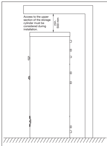
Illustr. 5.2 Minimum distance to the ceiling
