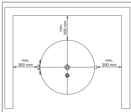
Illustr. 5.1 Minimum distances to the wall
