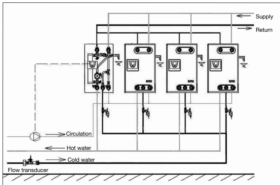
Illustr. 3: Installation example fresh water cascade consisting of:
