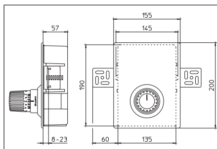
Illustr. 4.1 Dimensions
