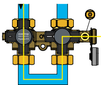
Fill and flush terminal unit
