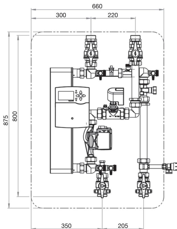
fig. 3.8: Dimensiones “Regumaq X-80” (frontal)
