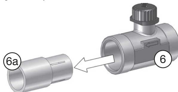
fig. 5.17: Retire el manguito interior
