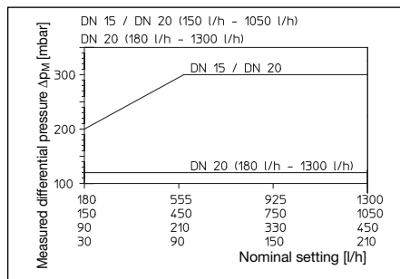
Illustr. 5.1 Differential pressure / Nominal setting
