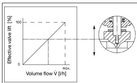
Illustr. 5.4 Characteristic line of the regulating unit "Cocon Q"
