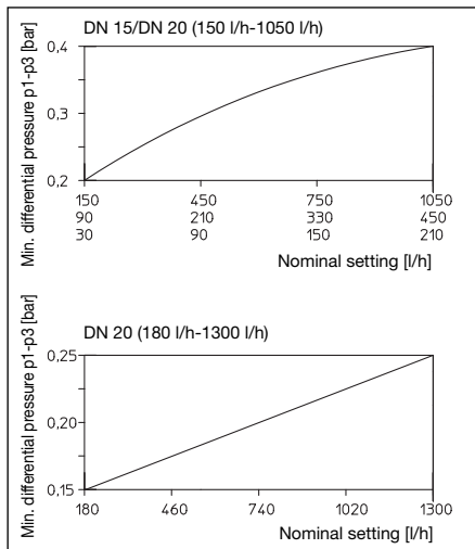
Illustr. 5.7 Differential pressure / Nominal setting
