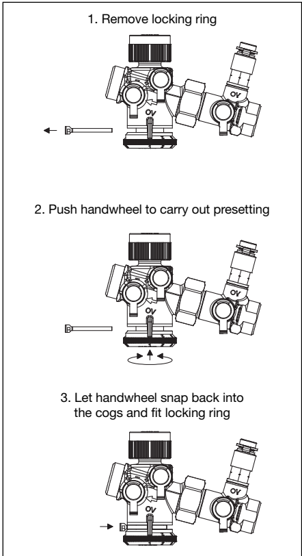
Illustr. 7.1 Setting of the flow rate
