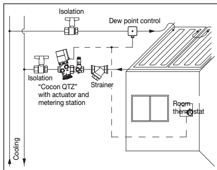
Illustr. 6.1 Two pipe system
