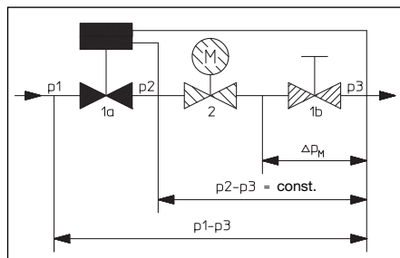
Illustr. 5.3 Function "Cocon QTZ"
