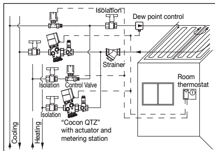
Illustr. 6.2 Four pipe system
