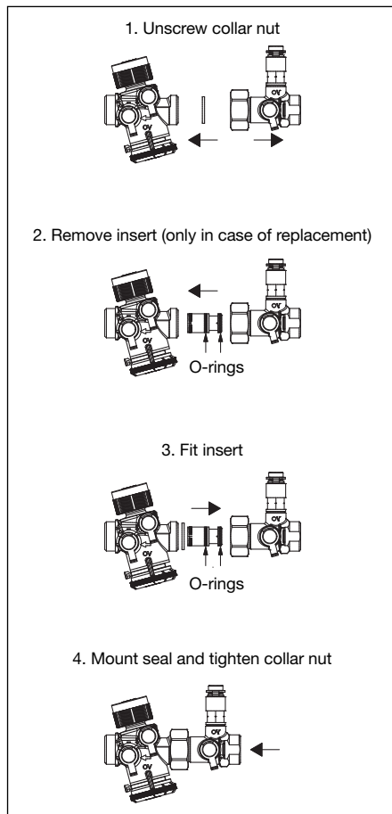
Illustr. 6.3 Replacement of metering station insert
