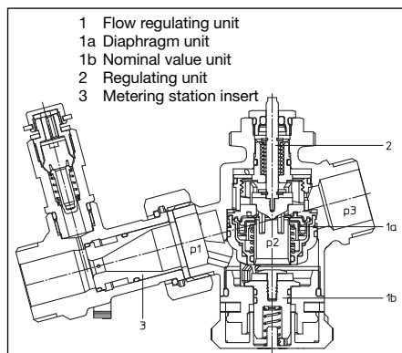
Illustr. 5.2 Construction "Cocon QTZ" with metering station
