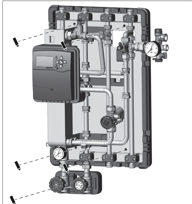
Illust. 28: Marking of the boreholes for fixing screws
