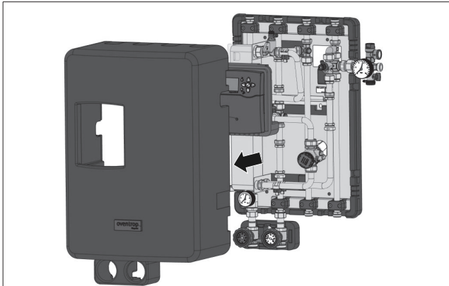
Illust. 26: Removal of the front insulation shell
