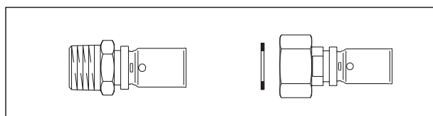
Connection system “Cofit P” for female and male threaded connection
