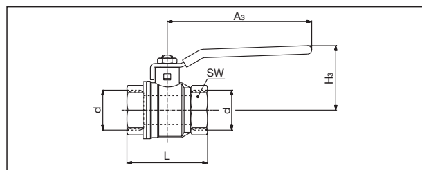
Dimensions item no. 1076002-32 (DN 8 up to DN 100) Lever made of galvanised steel with plastic coating
