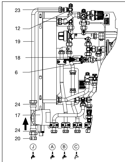
Illustr. 6.1 Installation
