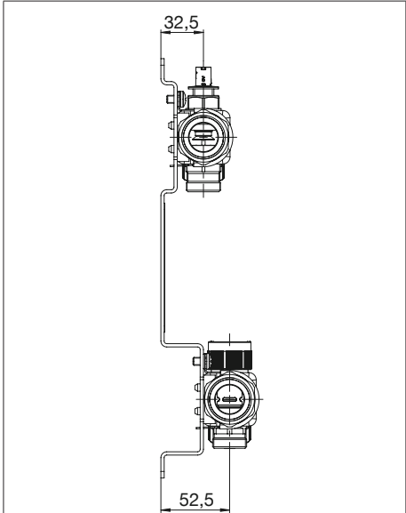
Illust. 7: Dimensions of the Multidis SFQ heating circuit distributor/collector lateral view
