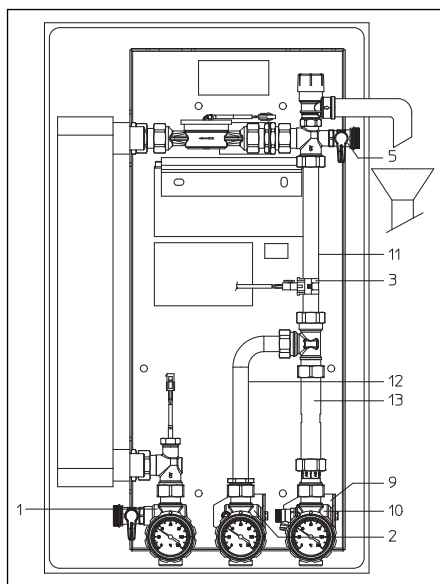
Illustr. 2: Fresh water station "Regumaq X-30" with piping set 1381080 (illustration secondary circuit)
