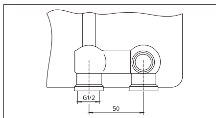
Illustr. 8 Distributor with G \frac{1}{2} female thread
