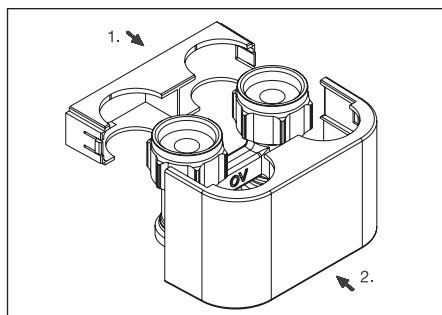
Illustr. 10 Installation of the design cover
