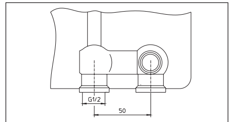
Abb. 8 Ventilgarnitur G \frac{1}{2} IG
