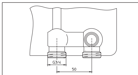
Illustr. 9 Distributor with G \frac{3}{4} male thread according to DIN EN 16313 (cone "Euro")
