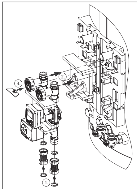
Illustr. 10 Installation of heating circuit group
