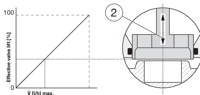
Fig. 5: Linear characteristic line of the regulating unit
