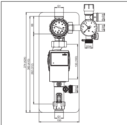
Illustr. 4.1 Pump circuit "Regusol PH-130 (180)" DN25
