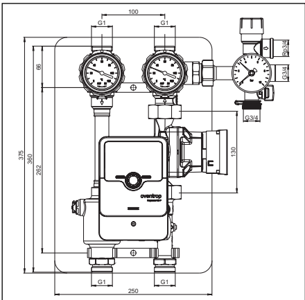
Illustr. 4.4 Solar station "Regusol ELH-130" DN25
