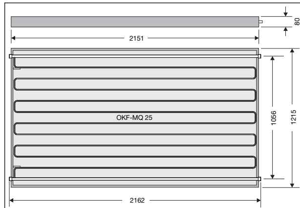
Illustr. 6: Dimensions
