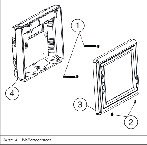
Illustr. 4: Wall attachment
