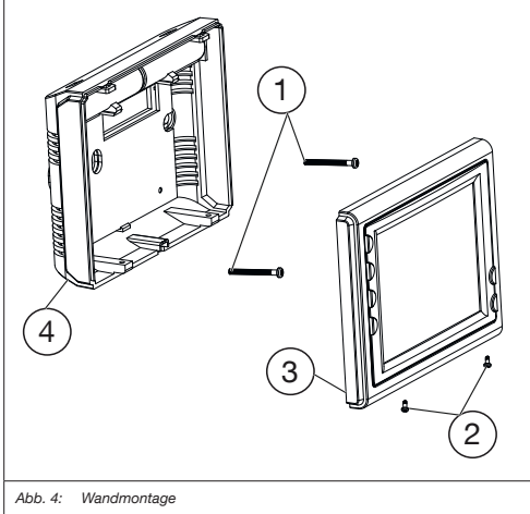
Abb. 4: Wandmontage
