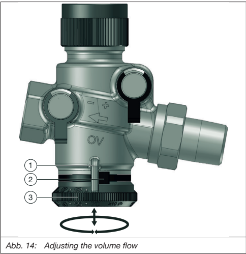
Abb. 14: Adjusting the volume flow
