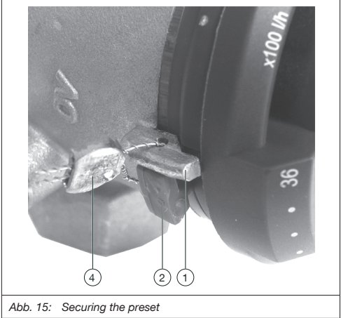
Abb. 15: Securing the preset
