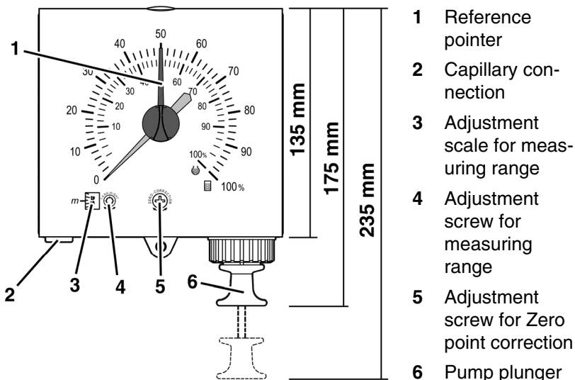
Fig. 1: Front view
