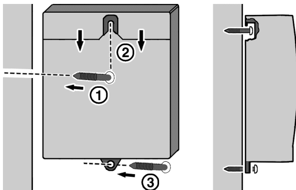
Figure 2: Montage mural
