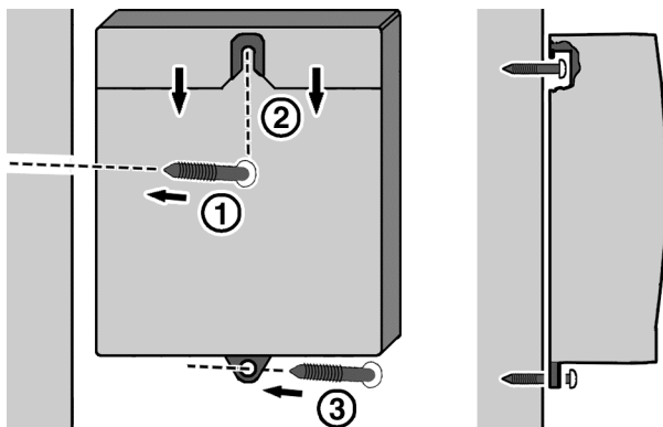
Fig. 2: Wall mounting
