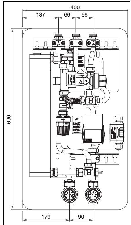
Illustr. 6.1: Installation, indications in mm
