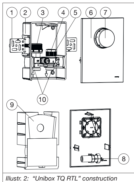
Illustr. 2: "Unibox TQ RTL" construction
