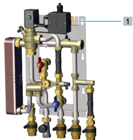
Abb. 12: Station erden
