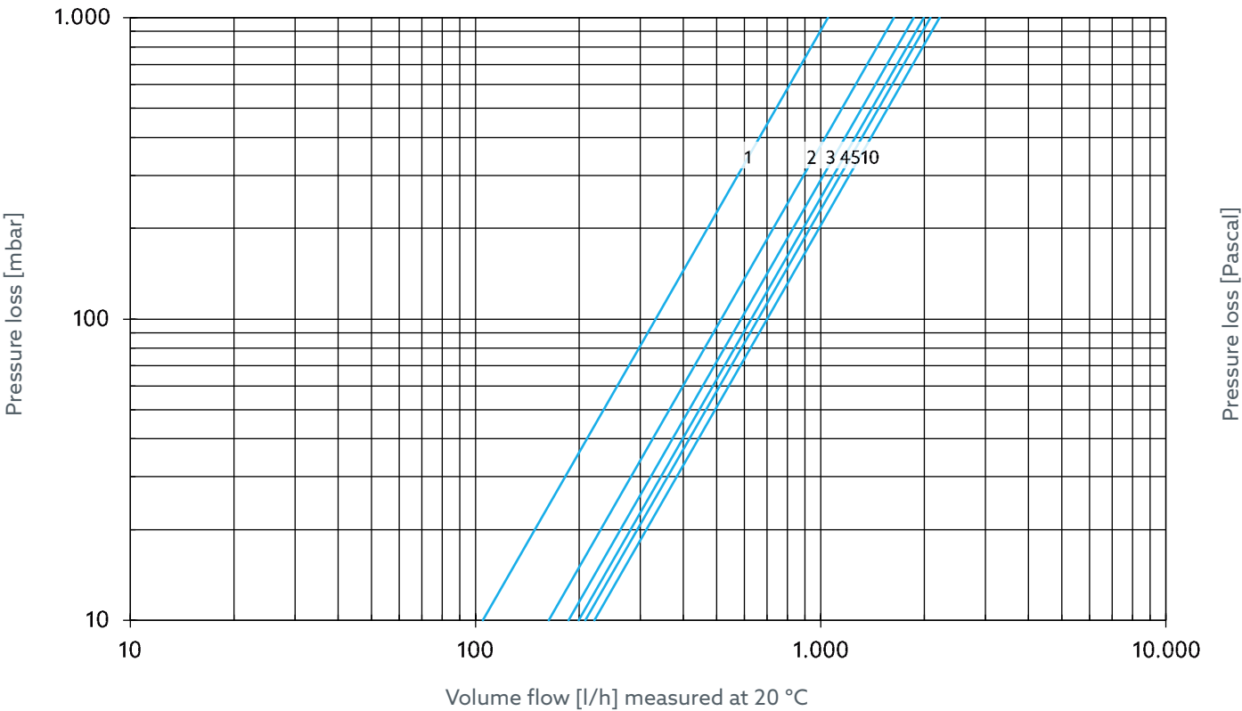
Fig. 16: Volume flow presetting DN 20
