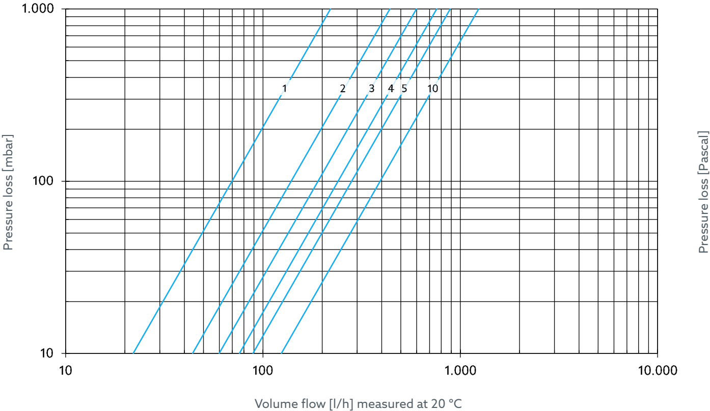
Fig. 15: Volume flow presetting DN 15
