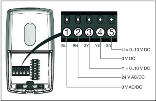
PIN assignment
