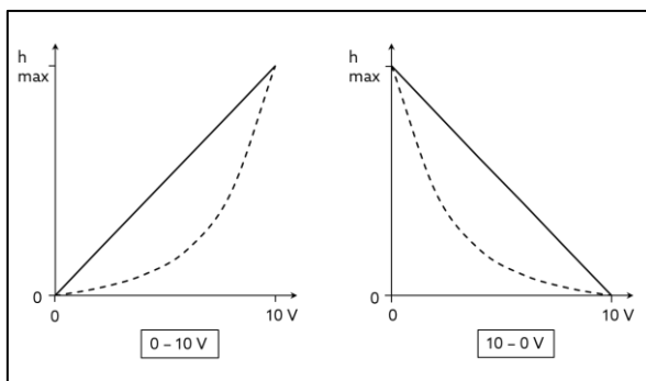
Characteristic line inversion DIP switch 7
