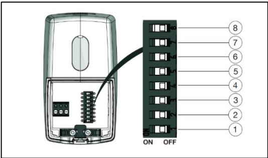
DIP switches
