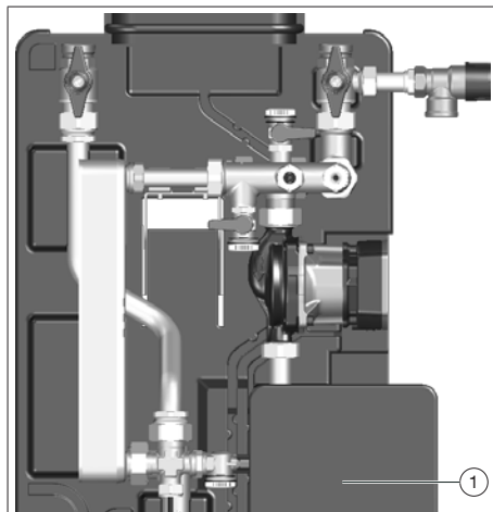
Illust. 4: Opening of the controller
