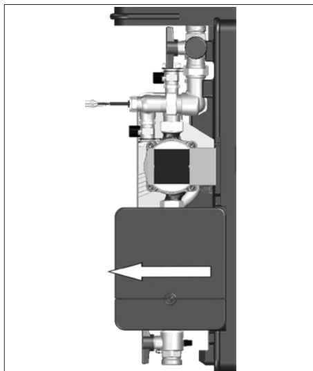
Illust. 2: Removal of the controller
