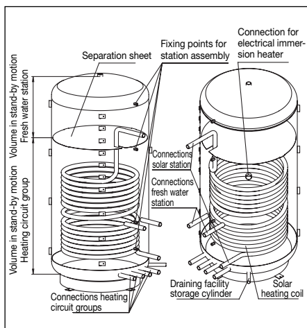
Illustr. 43 Functional illustrated section
