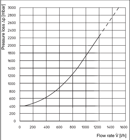
Pressure loss primary circuit (storage cylinder circuit) at maximum draw off operation
