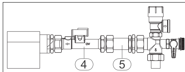
Illustr. 2: Installation Vortex flow sensor
