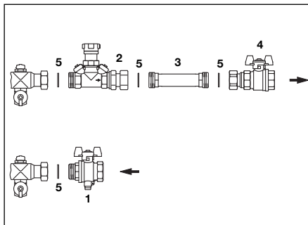
Illustr. 4: Heat meter connection set no. 1, straight pattern, extent of supply and location of components for right hand side connection
