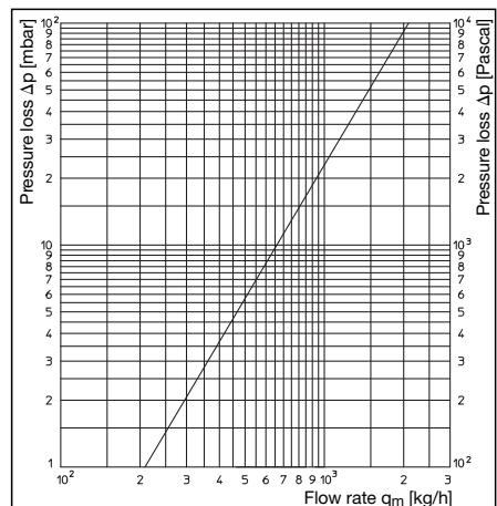
Chart 1: Pressure loss heat meter connection set no. 1, DN 20
