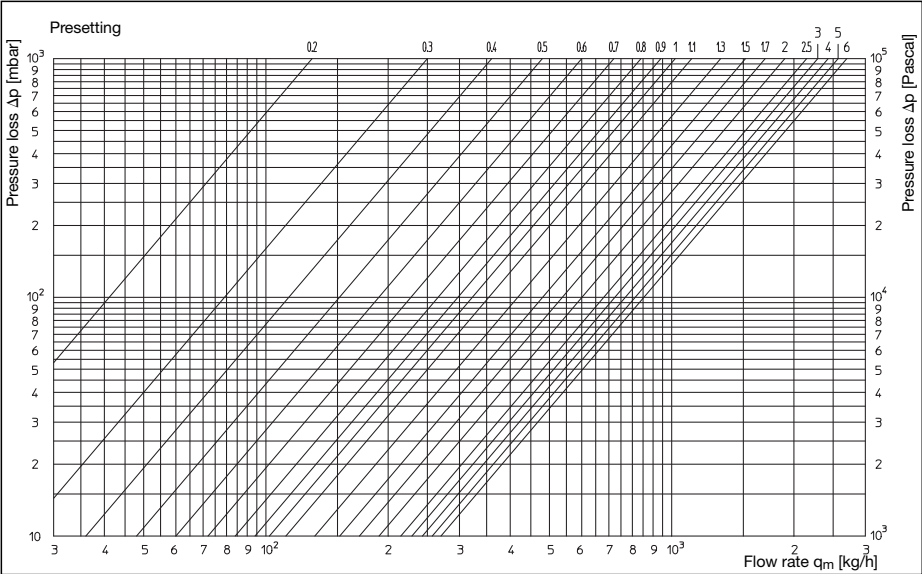
Chart 2: Pressure loss double regulating and commissioning valve “Hycocn VTZ” DN 20
