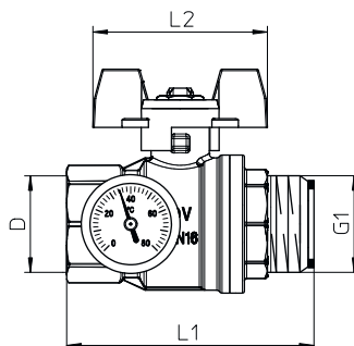
Illustr. 6: Dimensions of the ball valve
