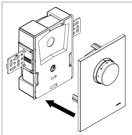
Illustr. 11: Positioning the cover plate with handwheel
