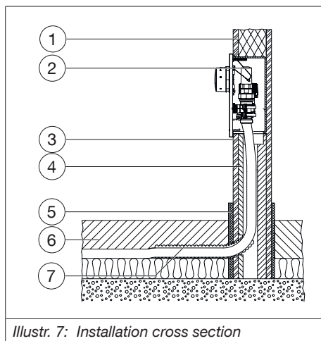
Illustr. 7: Installation cross section
