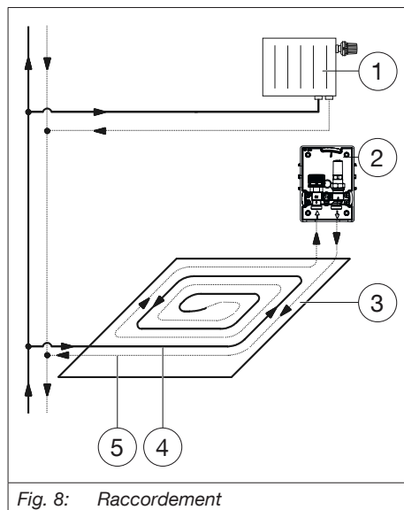
Fig. 8: Raccordement
