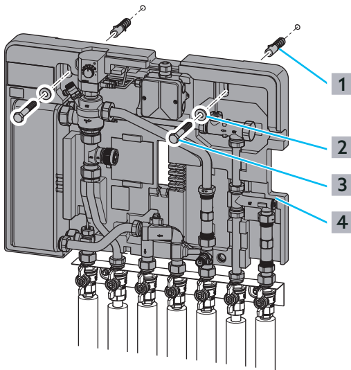
Abb. 18: Station montieren
