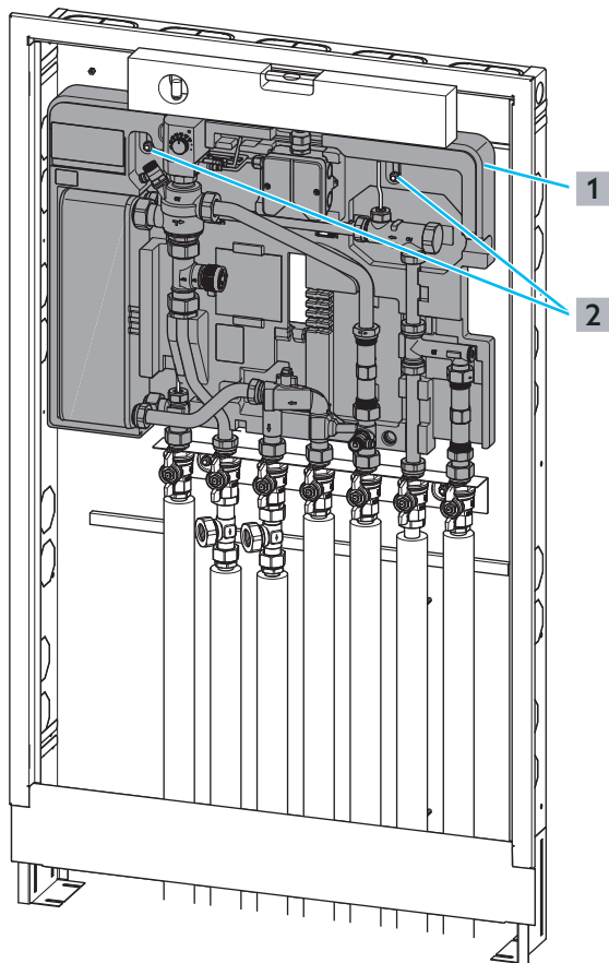
Abb. 14: Station montieren
