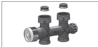
Illustr. 1 Fitting "Multiblock T", straight pattern G \frac{3}{4} collar nut x G \frac{3}{4} male thread
