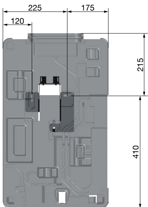
Fig. 8: Encombrements Regumaq X-25 support mural
