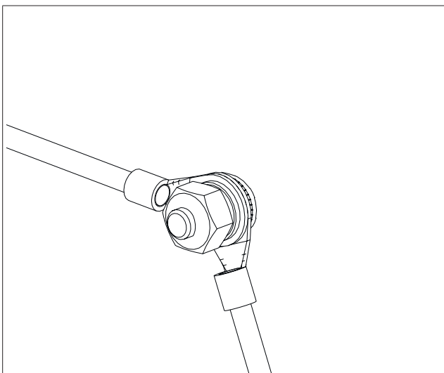
Illustr. 10: Central earthing point with connection to the equipotential bonding rail of the building and to the door of the surface-mounted cabinet
