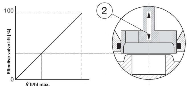
Fig. 5: Linear characteristic line of the regulating unit
