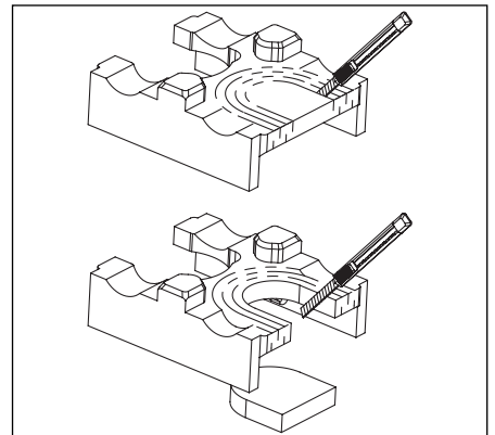
Illustr. 5.6 Insertion block with cutting for heat meter
